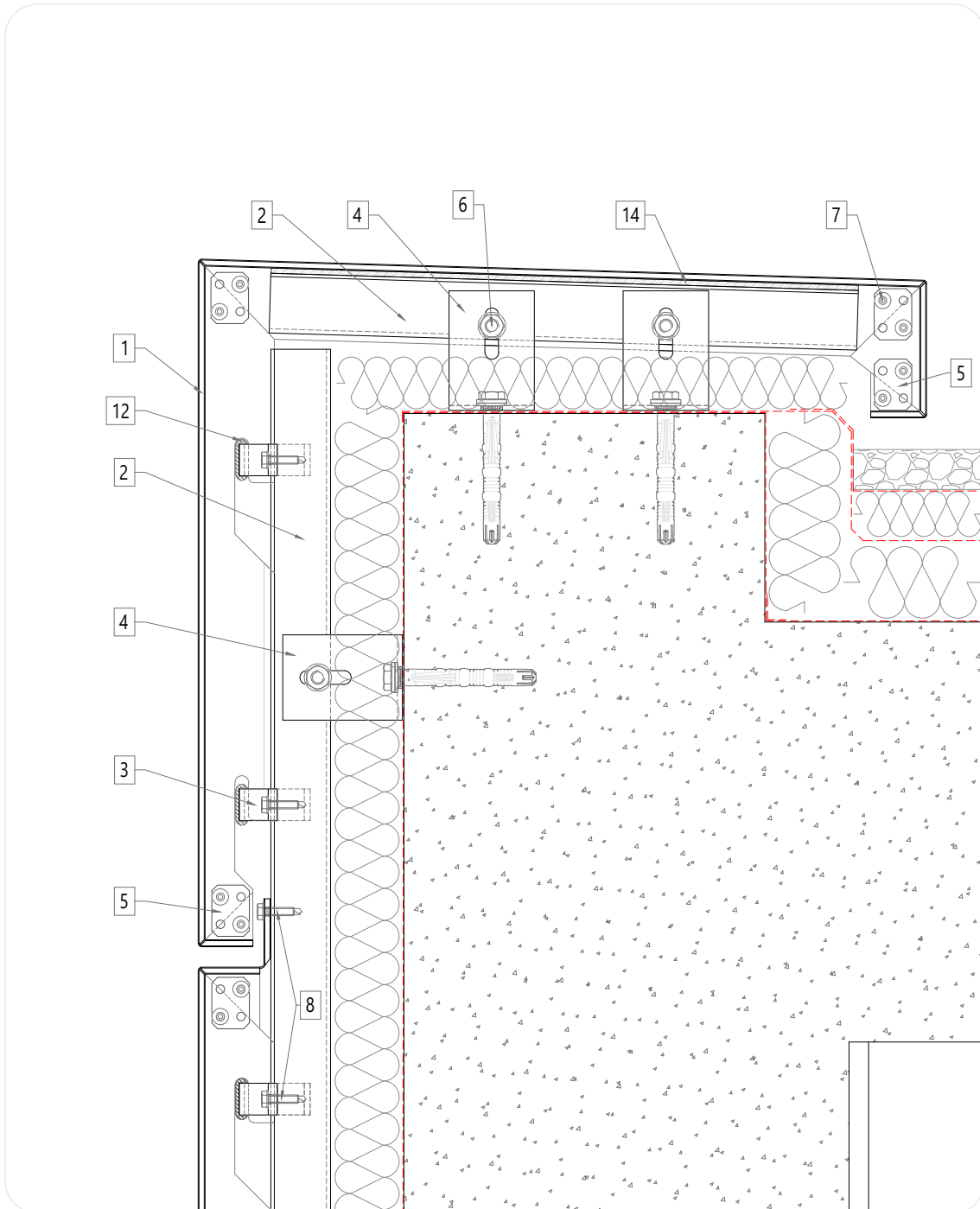
07. Parapet detail
