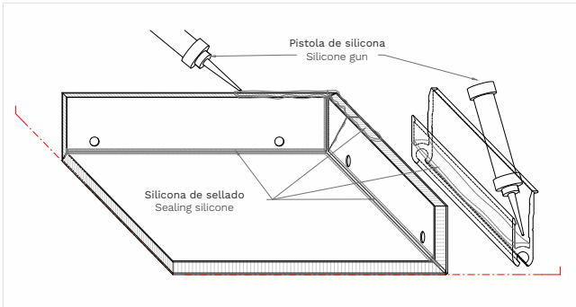
Sealing silicone is also applied to cassette corners and the inside of the LT-4 profiles along its entire length.
