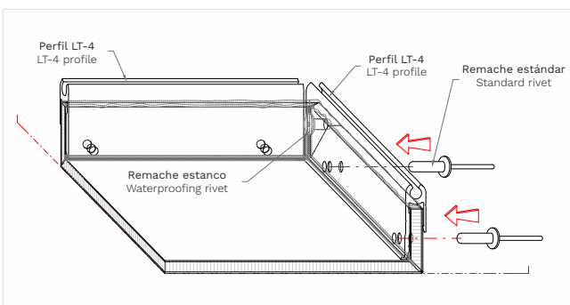
Fixing of the standard rivets.
