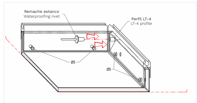
Fixing of the waterproofing rivets.
