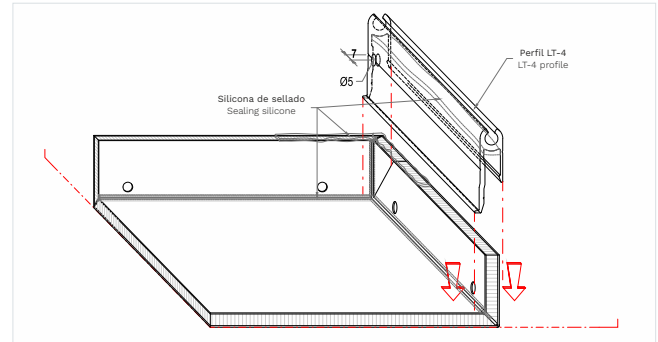
Placement to the LT-4 profile. Before a drill should be done in both sides of the profile.
