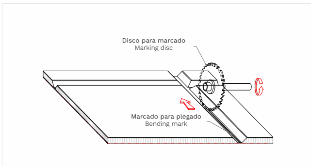
To achieve an accurate 90° bending, it is necessary to mark the middle of the lower side of the routing.
